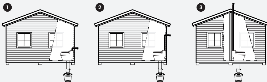
Options for ventilation. The Villa models are installed with up to six meters of ventilation pipes and three 90-degree bends. Ventilation kit is not included.
